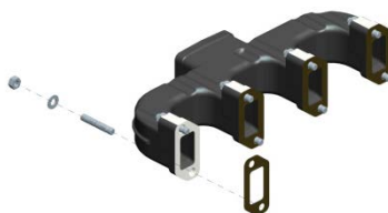
Exhaust Manifold
