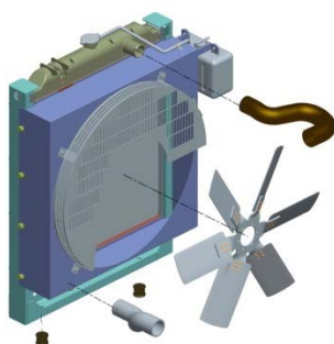
Radiator Assembly
