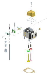
Cylinder Head
