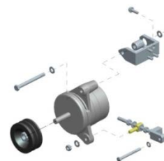
Alternator
