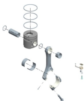
Connecting Rod & Piston
