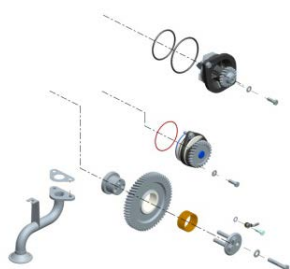
Gear Train
