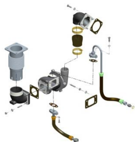
Turbocharger Assembly
