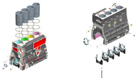
Crank Case
