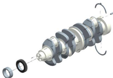
Crankshaft
