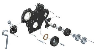
Front Cover
